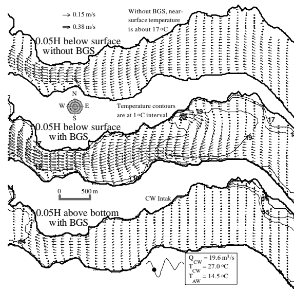
Fig. 10. Simulated peak ebb flows and temperatures at summer conditions with T_{AW} \approx 14.5 °C, where upper panel represents the near-surface flows without the BGS in operation, and middle and lower panels respectively represent the near-surface and near-bottom flows and temperatures with the BGS in operation under the conditions of Q_{CW} = 19.6 m 3 /s, U_1 = 0.5 m/s, U_2 = 1.5 m/s, and T_{CW} = 27 °C.
