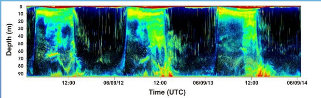
Backscatter signal over 3 days from a 200 kHz inverted echo sounder mounted on the VENUS array in Saanich Inlet, BC.
